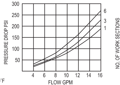
OPEN CENTER PRESSURE DROP P-A-B-T
